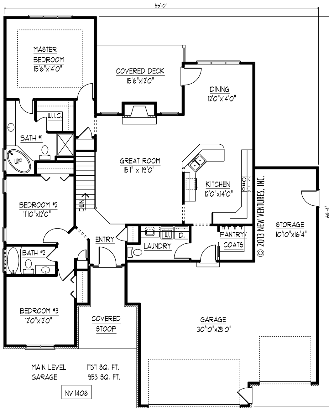
MAIN LEVEL FLOOR PLAN
