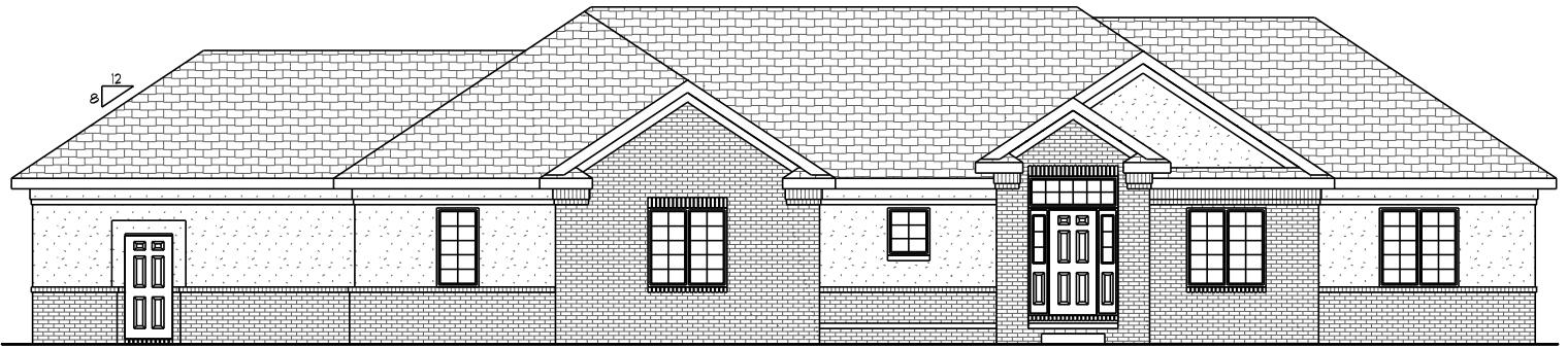
FRONT ELEVATION
