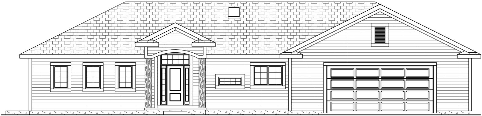
FRONT ELEVATION NV29815
