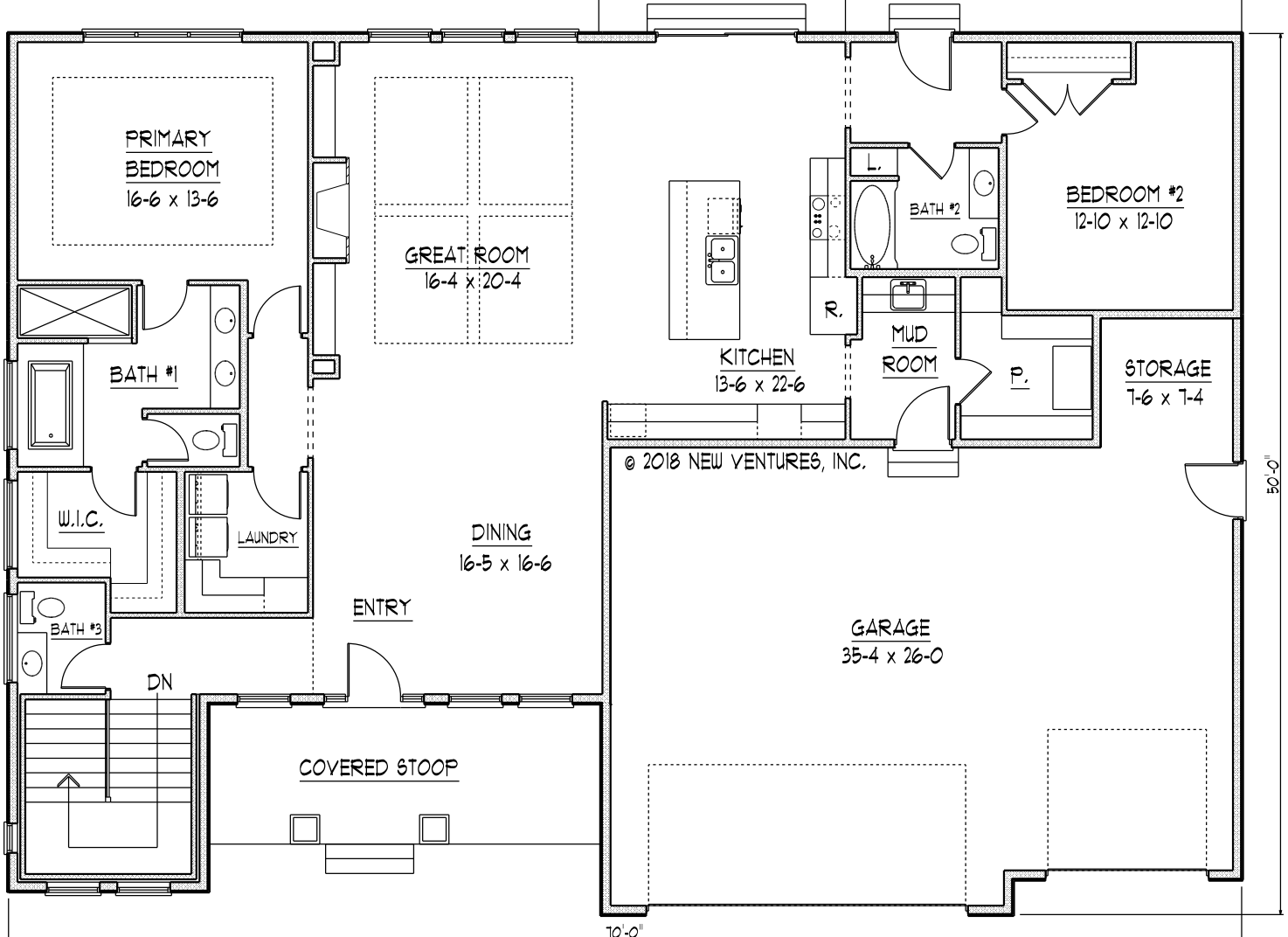
MAIN LEVEL FLOOR PLAN NV26219
