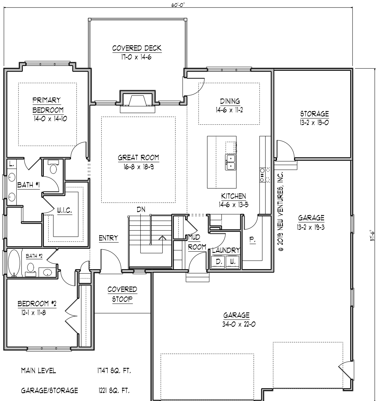
MAIN LEVEL FLOOR PLAN NY25119
