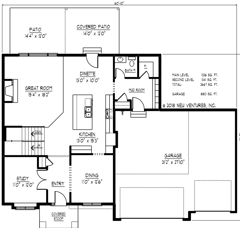
MAIN LEVEL FLOOR PLAN NVO9115
