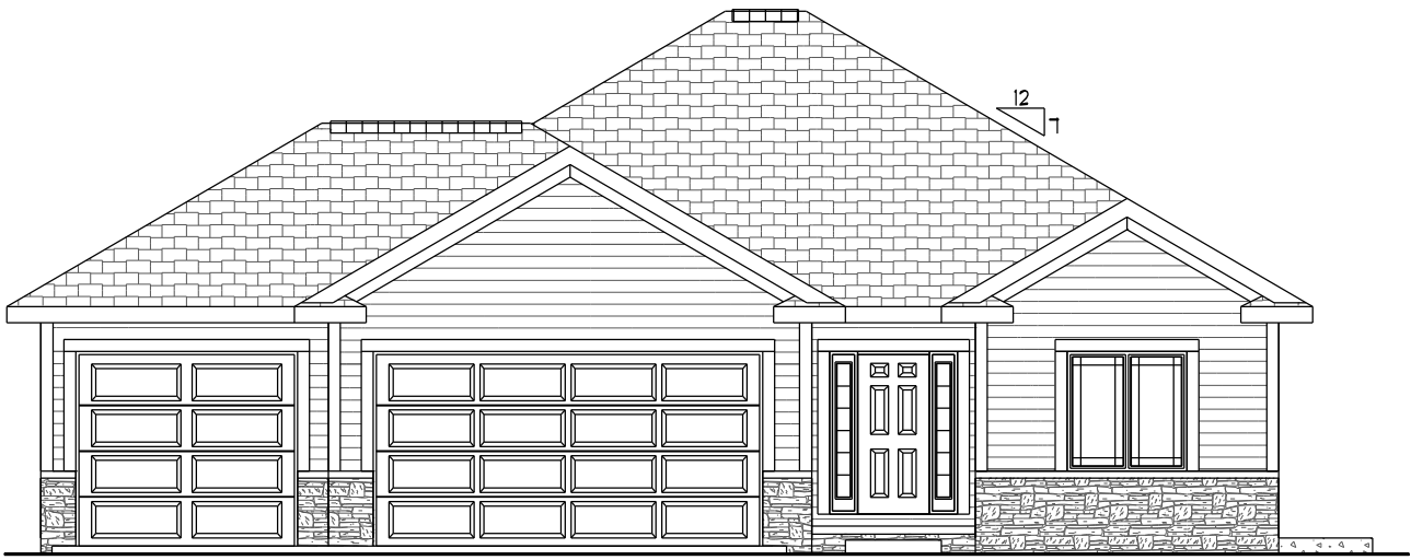
FRONT ELEVATION
