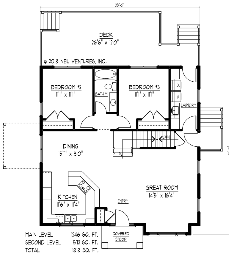
MAIN LEVEL FLOOR PLAN NV07115
