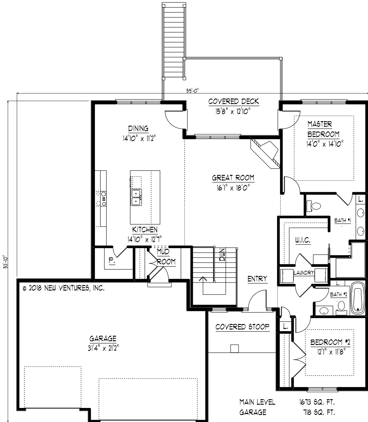
MAIN LEVEL FLOOR PLAN NV06816
