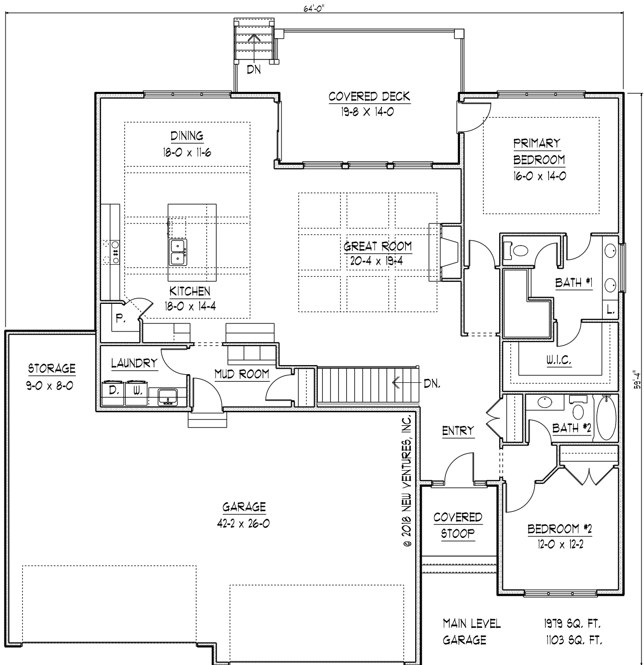
MAIN LEVEL FLOOR PLAN NV05419
