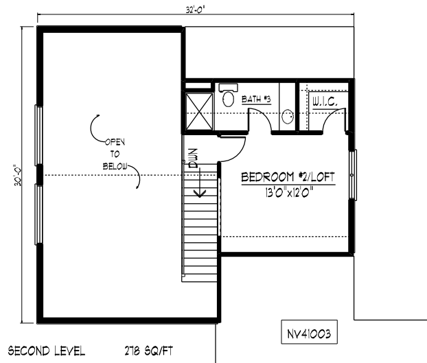
SECOND LEVEL FLOOR PLAN
