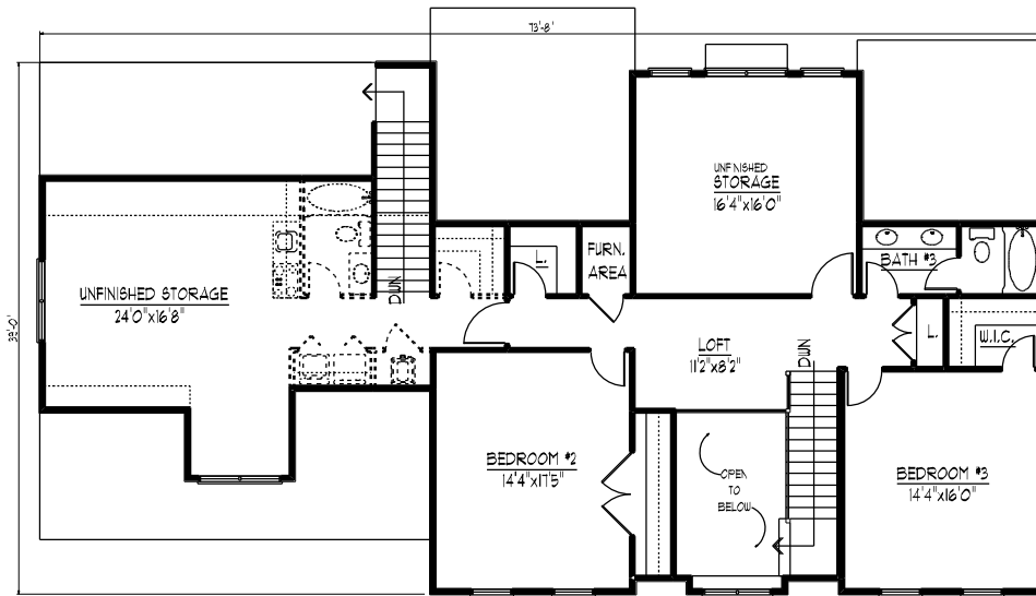
SECOND LEVEL FLOOR PLAN
