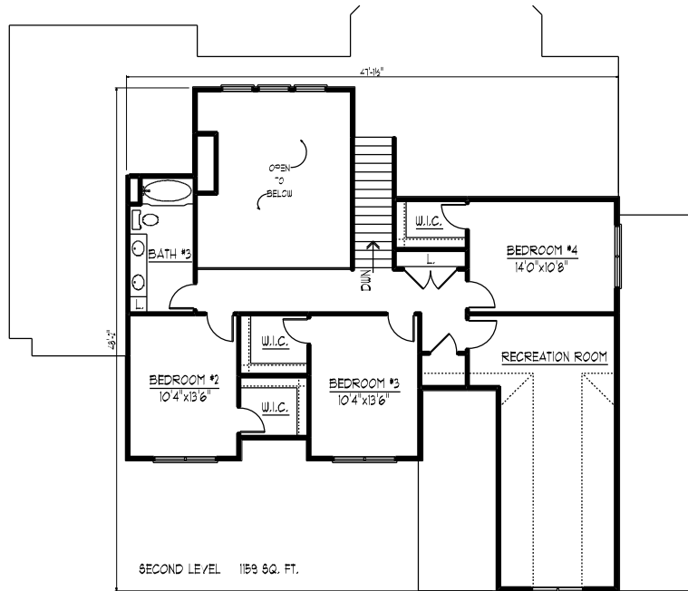
SECOND LEVEL FLOOR PLAN
