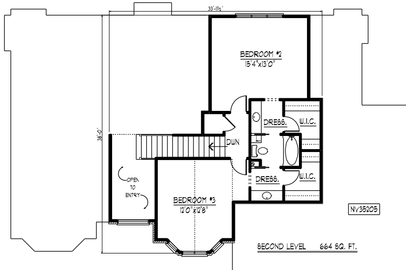
SECOND LEVEL FLOOR PLAN
