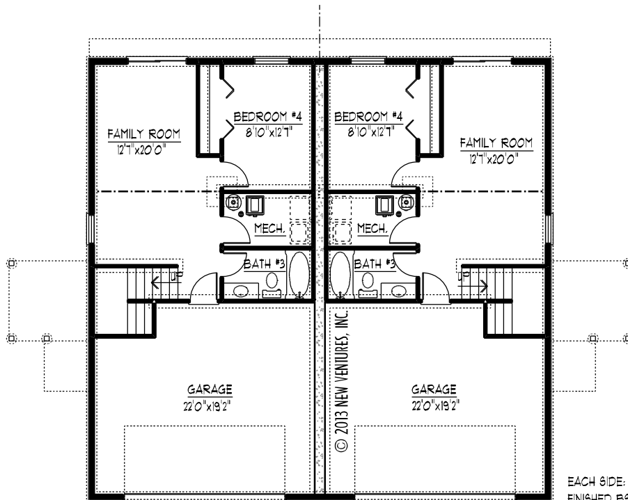
FOUNDATION PLAN
