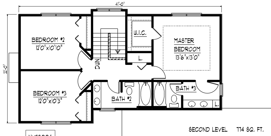
SECOND LEVEL FLOOR PLAN
