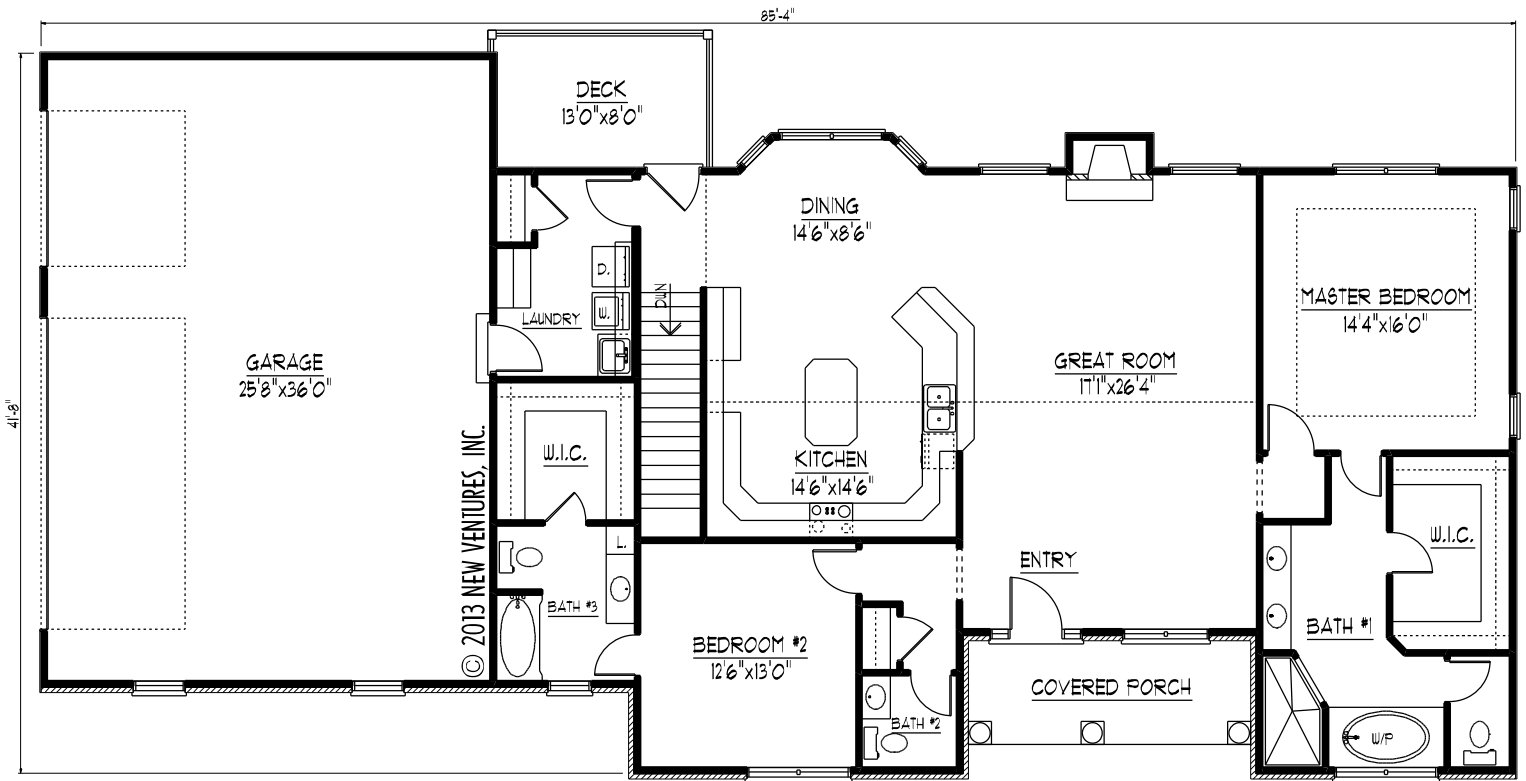
MAIN LEVEL FLOOR PLAN
