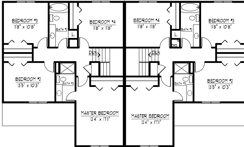
SECOND LEVEL FLOOR PLAN
