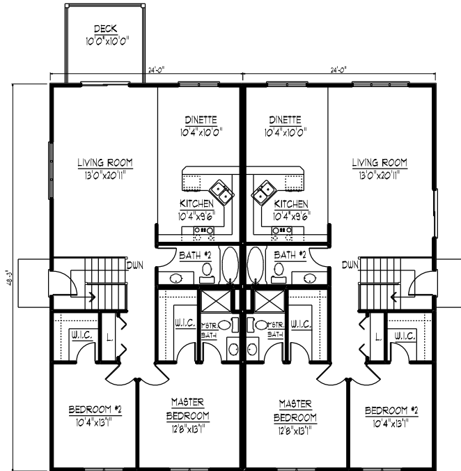
MAIN LEVEL FLOOR PLAN
