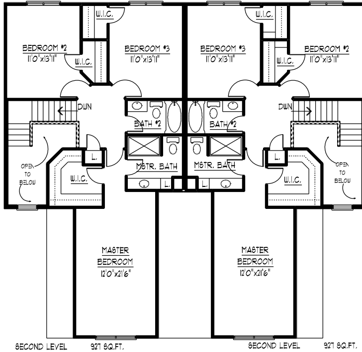
SECOND LEVEL FLOOR PLAN NV29806
