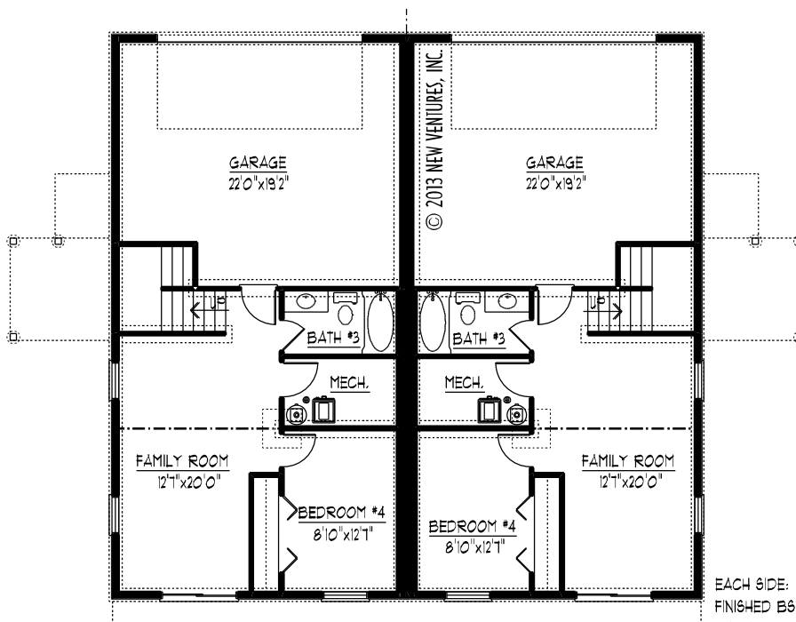
FOUNDATION PLAN
