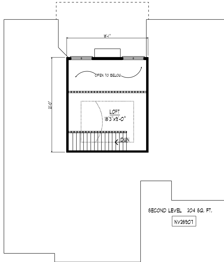
SECOND LEVEL FLOOR PLAN
