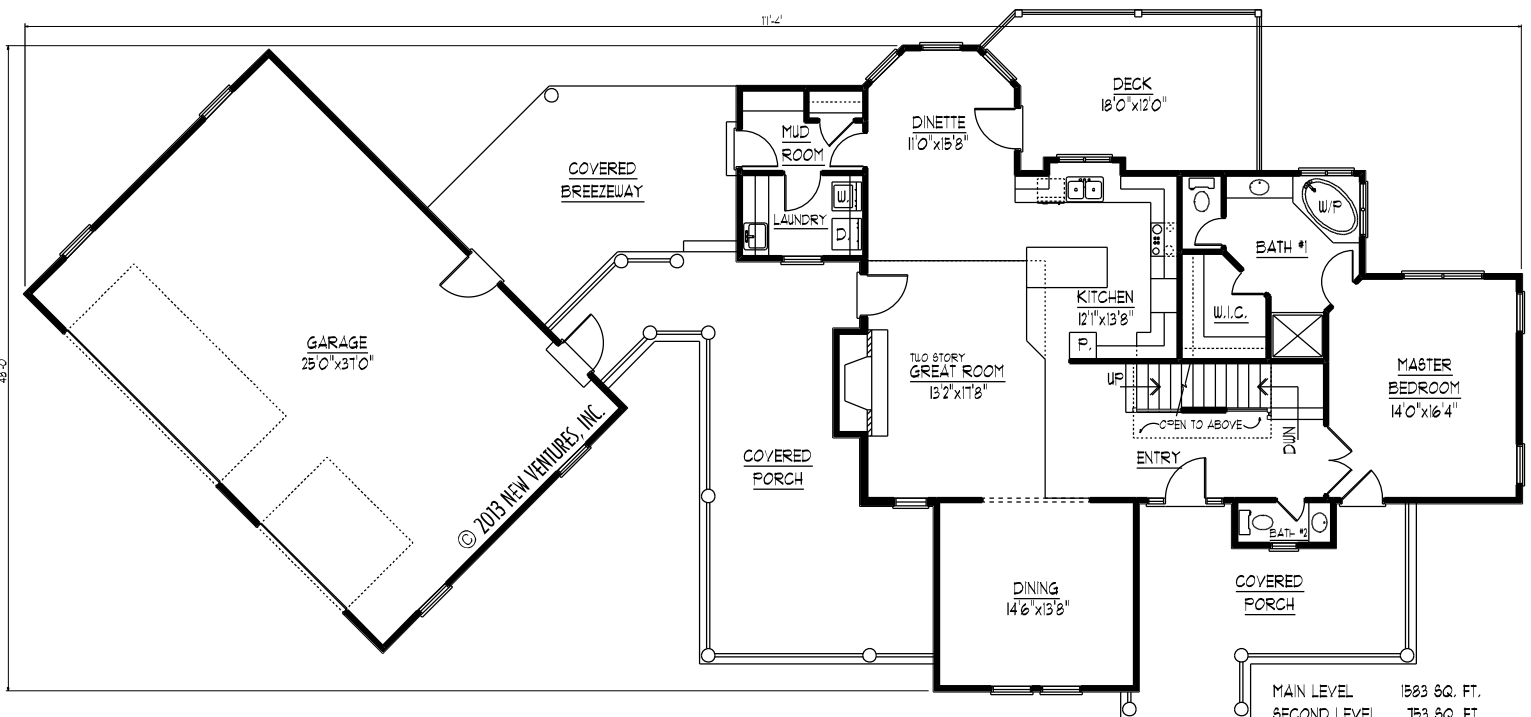
MAIN LEVEL FLOOR PLAN
