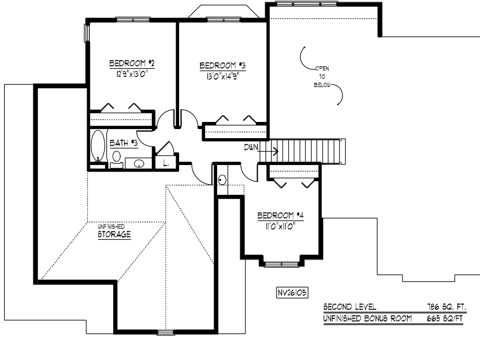
SECOND LEVEL FLOOR PLAN
