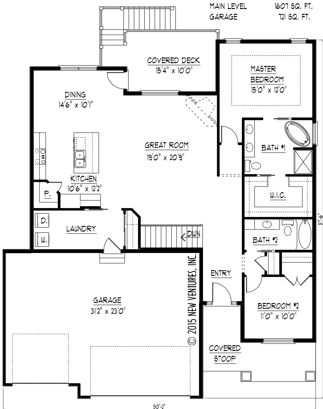
MAIN LEVEL FLOOR PLAN NV25012
