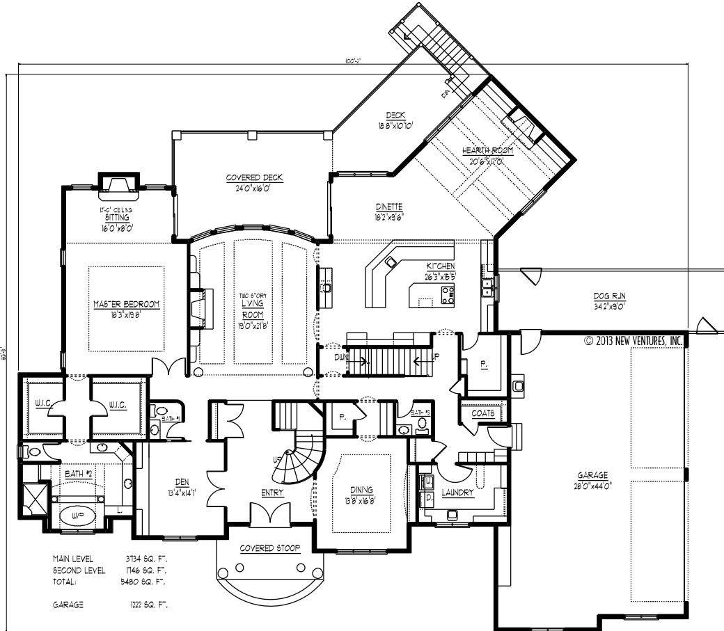
MAIN LEVEL FLOOR PLAN NV24603
