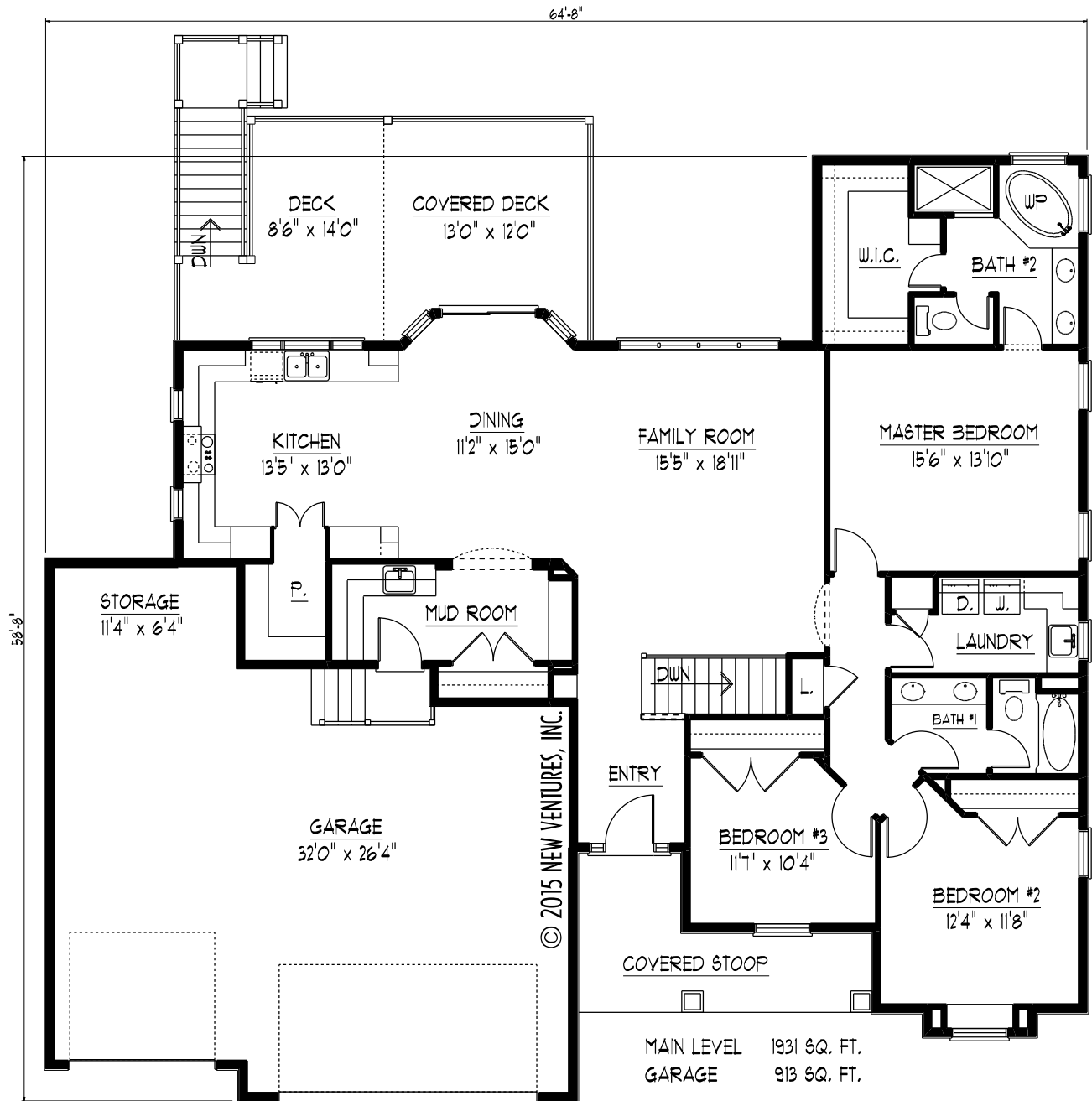
MAIN LEVEL FLOOR PLAN NV23412
