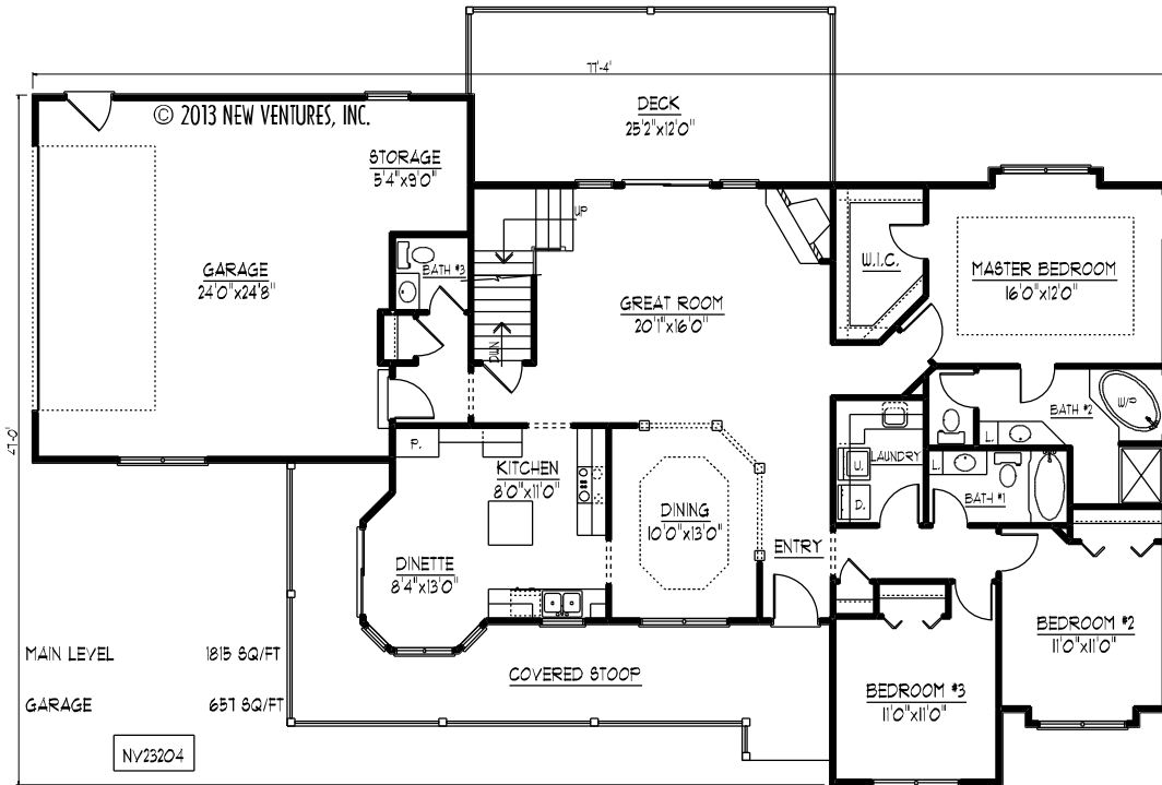
MAIN LEVEL FLOOR PLAN
