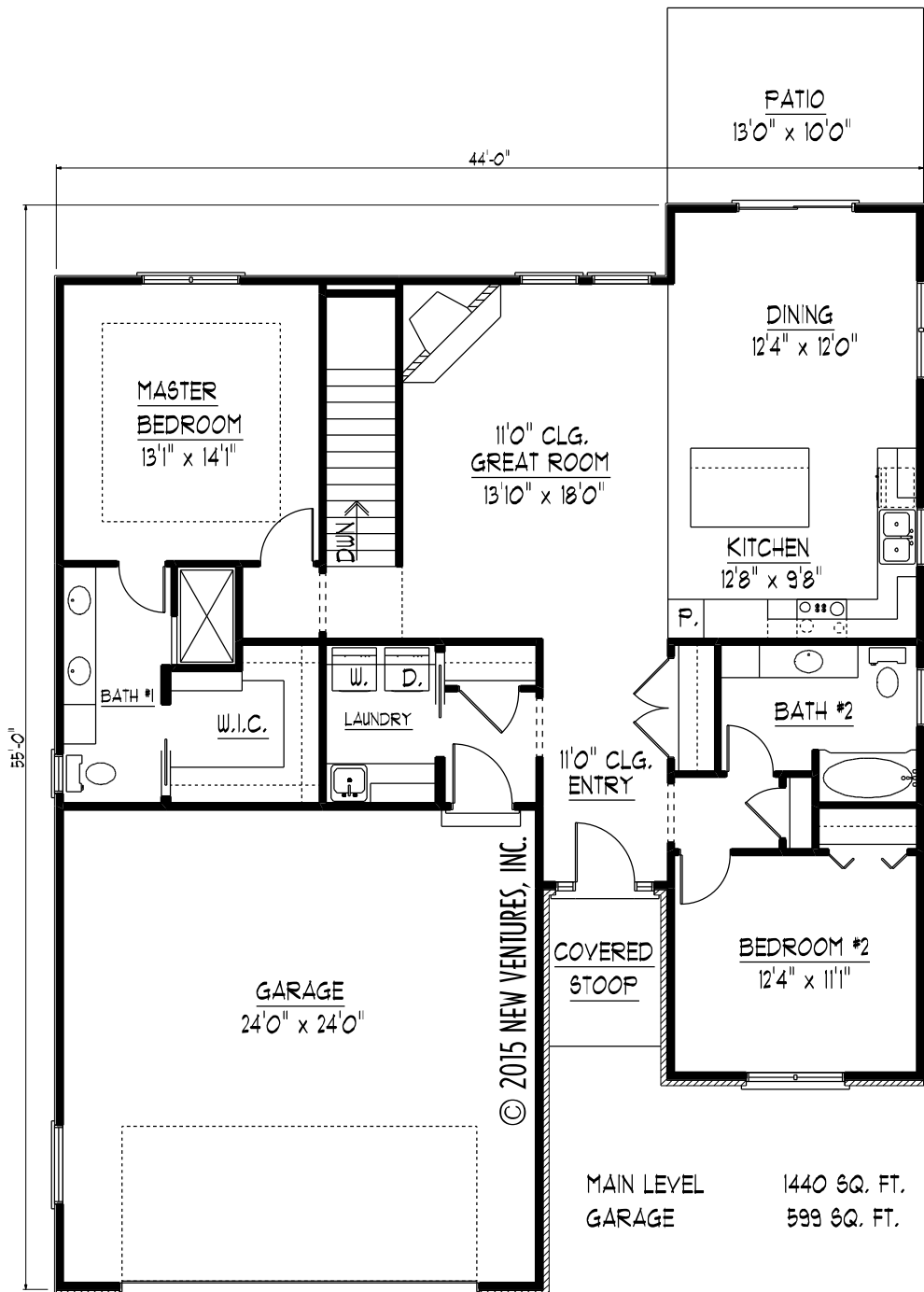
MAIN LEVEL FLOOR PLAN NV23112
