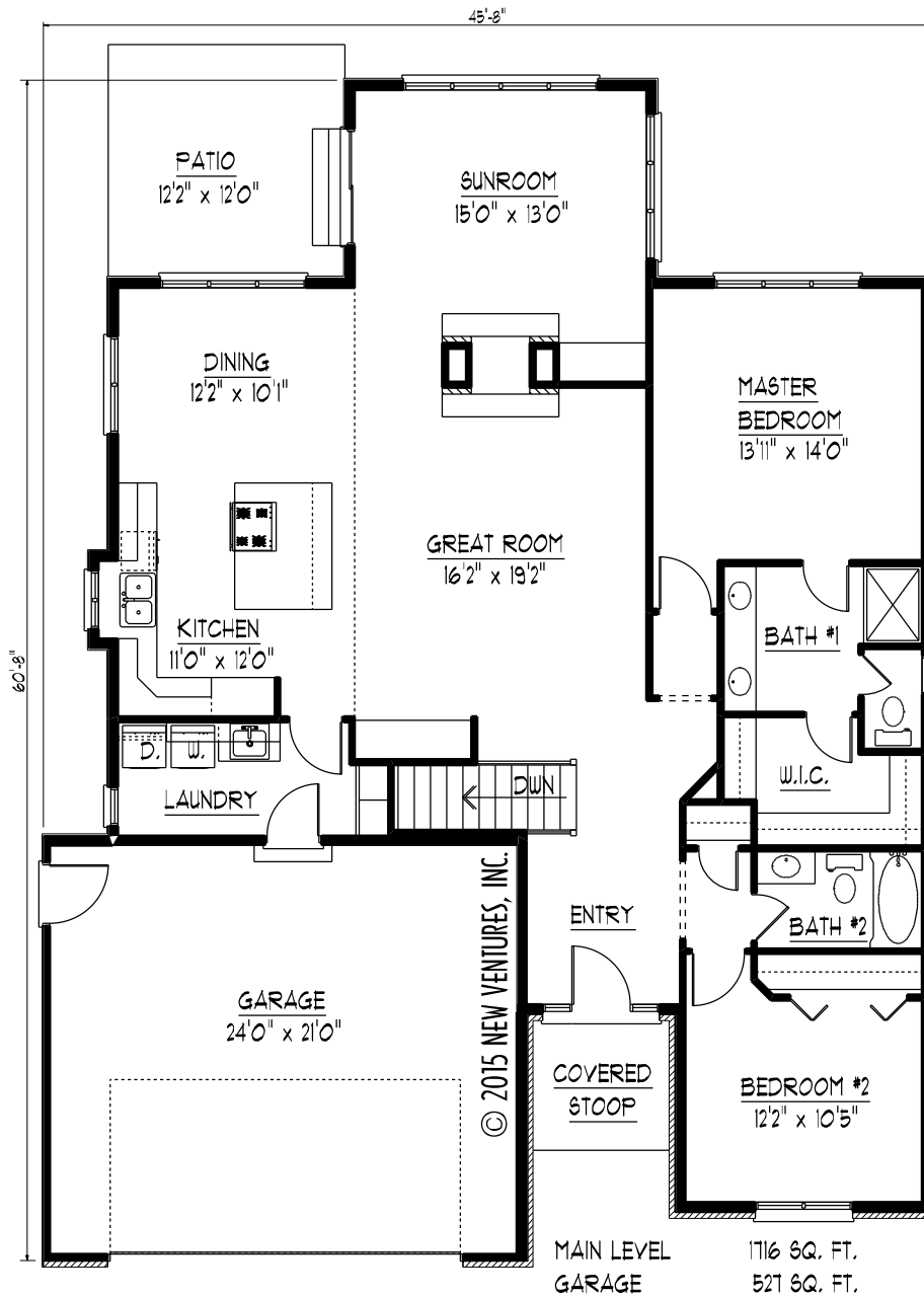
MAIN LEVEL FLOOR PLAN
