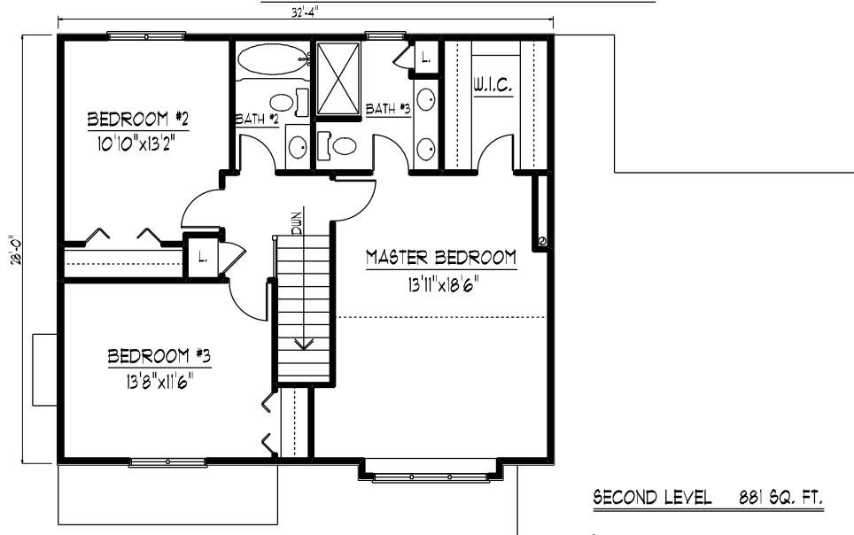
SECOND LEVEL FLOOR PLAN
