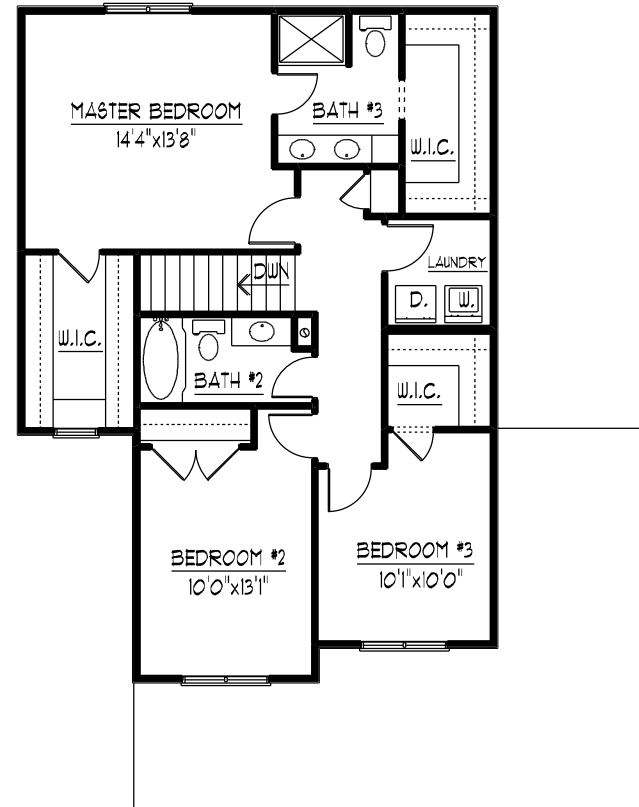
SECOND LEVEL FLOOR PLAN
