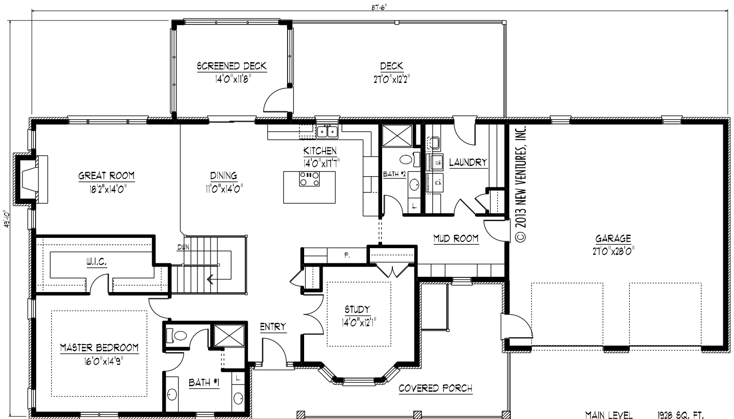
MAIN LEVEL FLOOR PLAN
