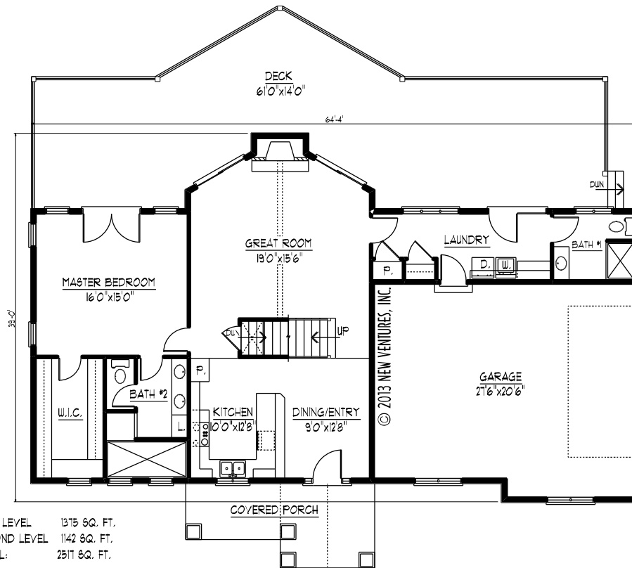
MAIN LEVEL FLOOR PLAN NV20805
