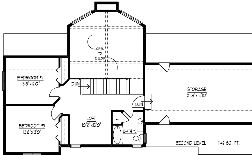
SECOND LEVEL FLOOR PLAN
