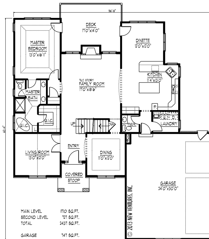
MAIN LEVEL FLOOR PLAN NV20505
