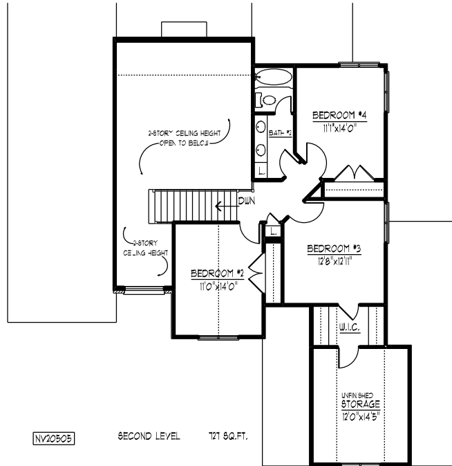
SECOND LEVEL FLOOR PLAN
