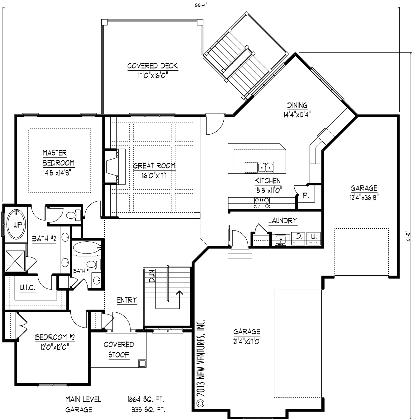
MAIN LEVEL FLOOR PLAN NV20110
