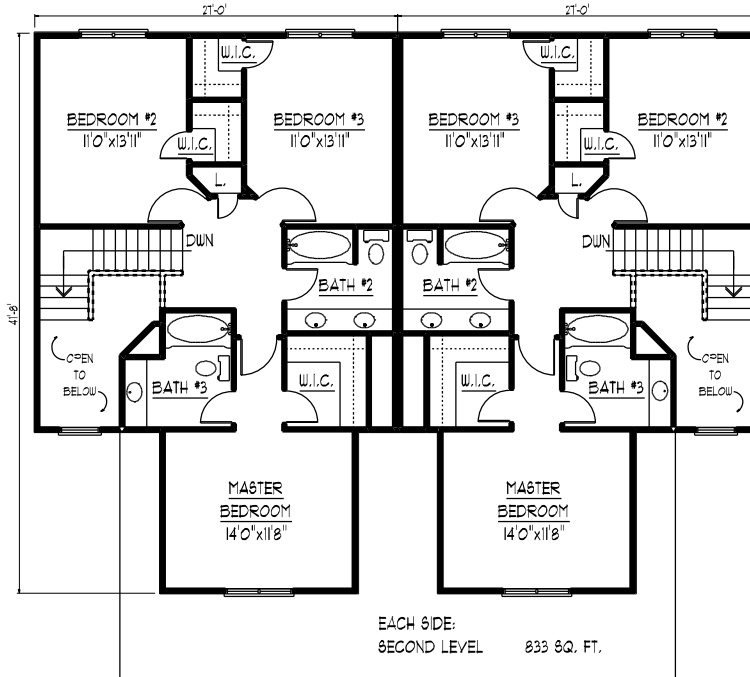
SECOND LEVEL FLOOR PLAN
