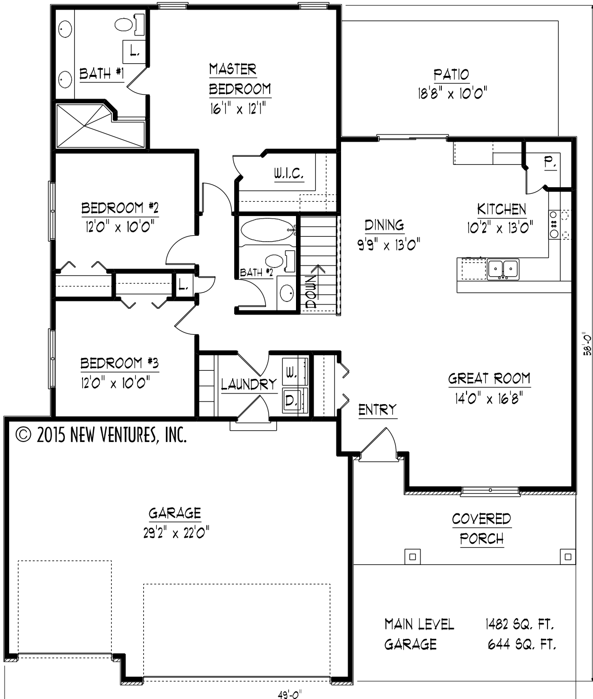
MAIN LEVEL FLOOR PLAN NV17112
