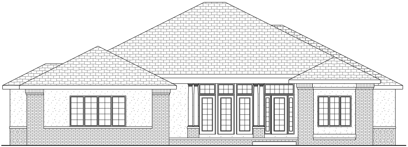
FRONT ELEVATION
