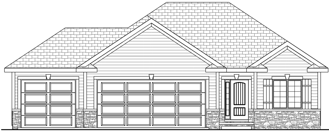
FRONT ELEVATION NY17113
