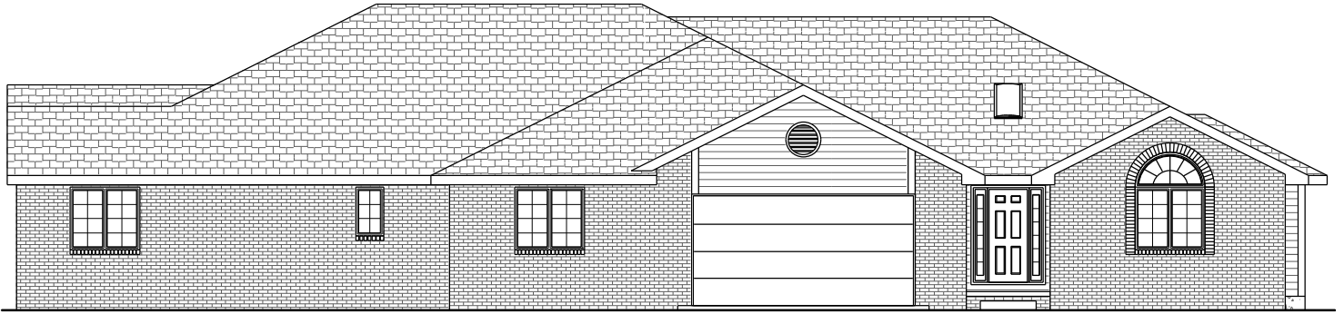
FRONT ELEVATION
