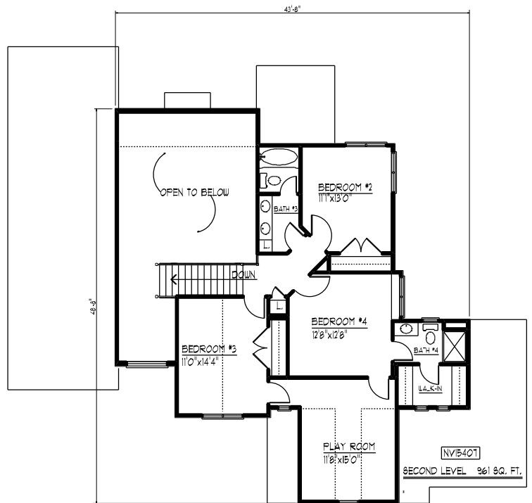
SECOND LEVEL FLOOR PLAN
