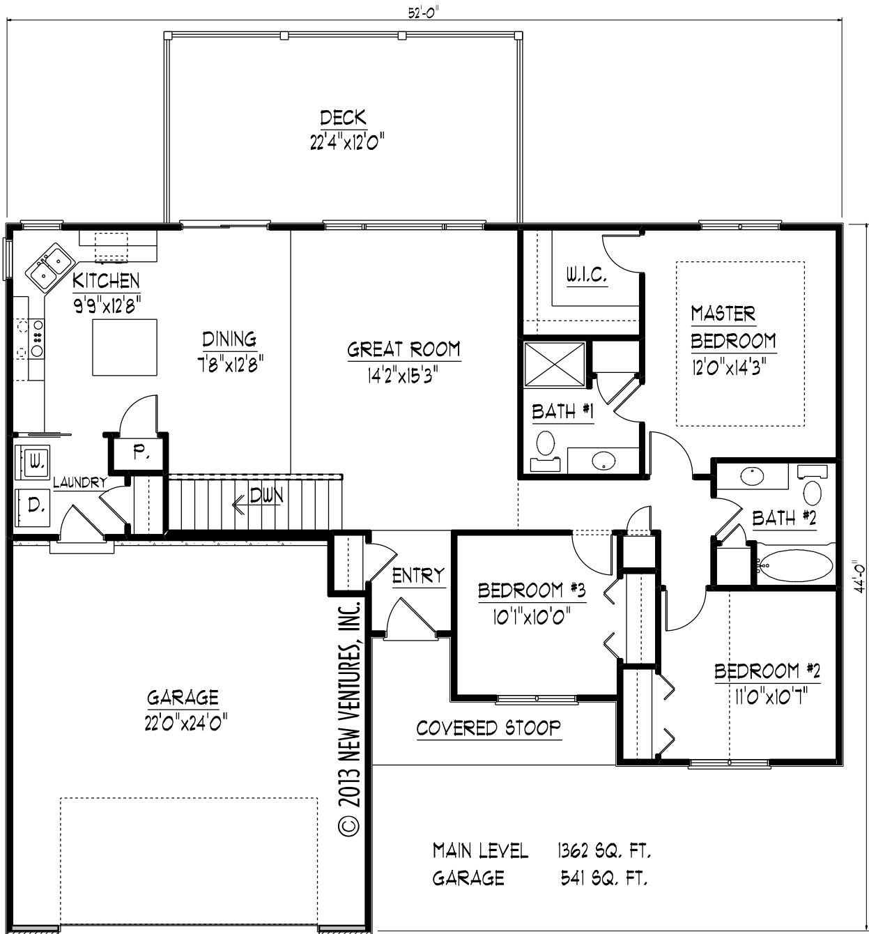
MAIN LEVEL FLOOR PLAN
