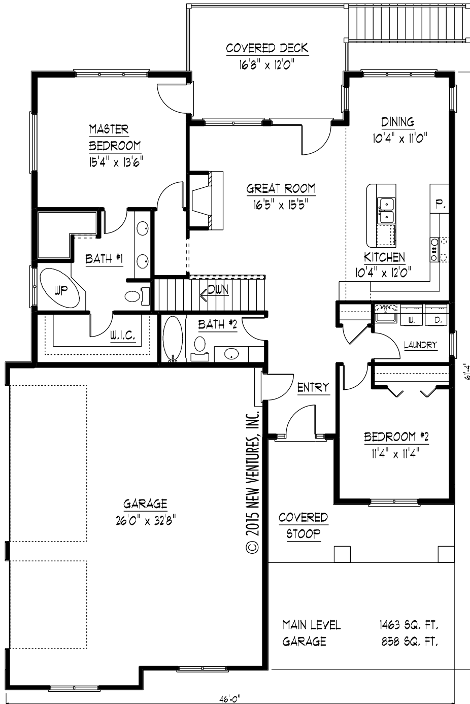
MAIN LEVEL FLOOR PLAN NV15012
