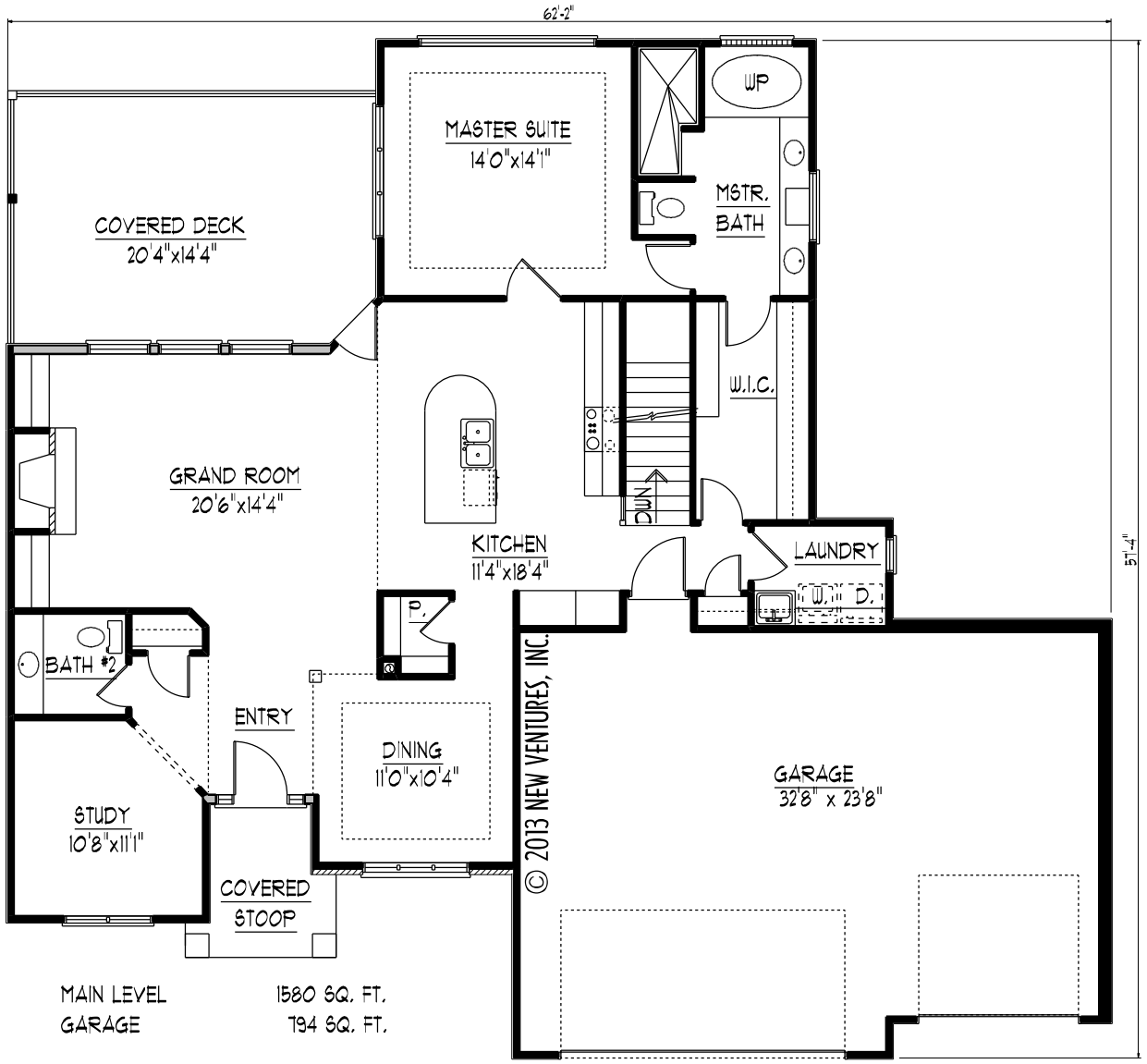
MAIN LEVEL FLOOR PLAN NV13509
