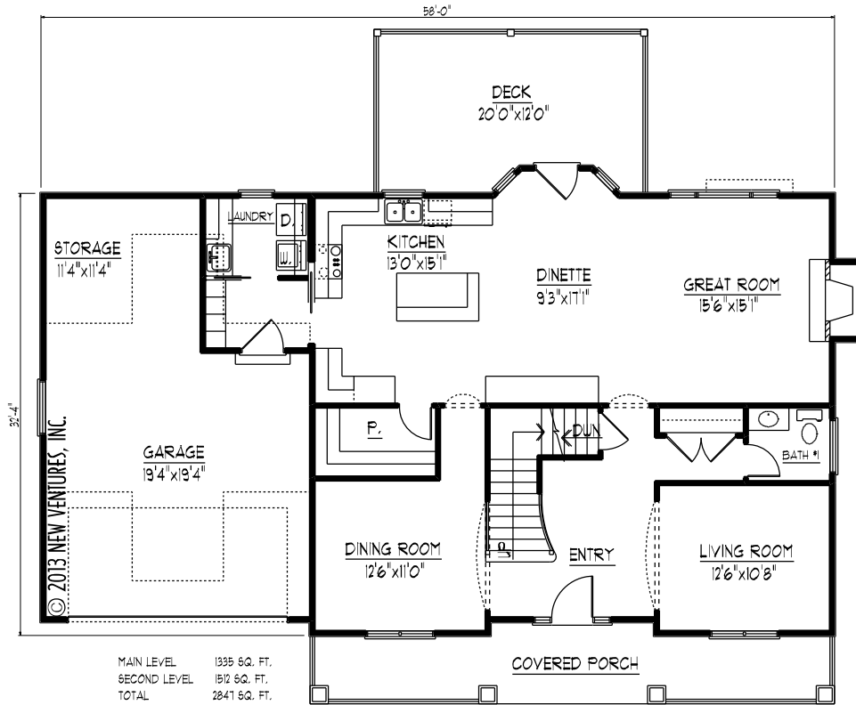
MAIN LEVEL FLOOR PLAN NV12308
