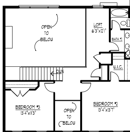
SECOND LEVEL FLOOR PLAN
