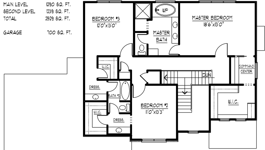
SECOND LEVEL FLOOR PLAN
