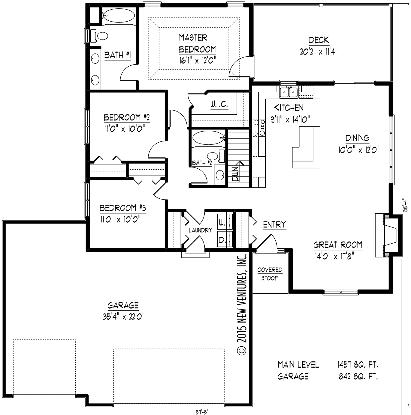
MAIN LEVEL FLOOR PLAN NV09913
