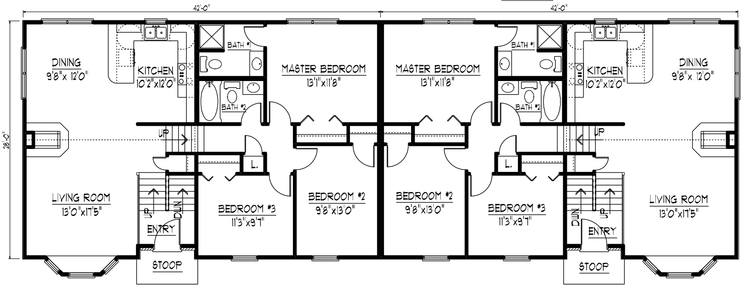
MAIN LEVEL FLOOR PLAN
